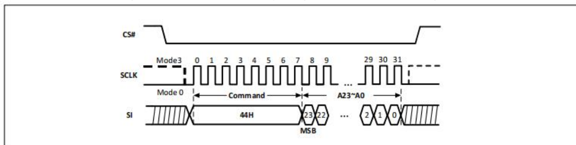
Figure-46. Erase Security Register Sequence Diagram
