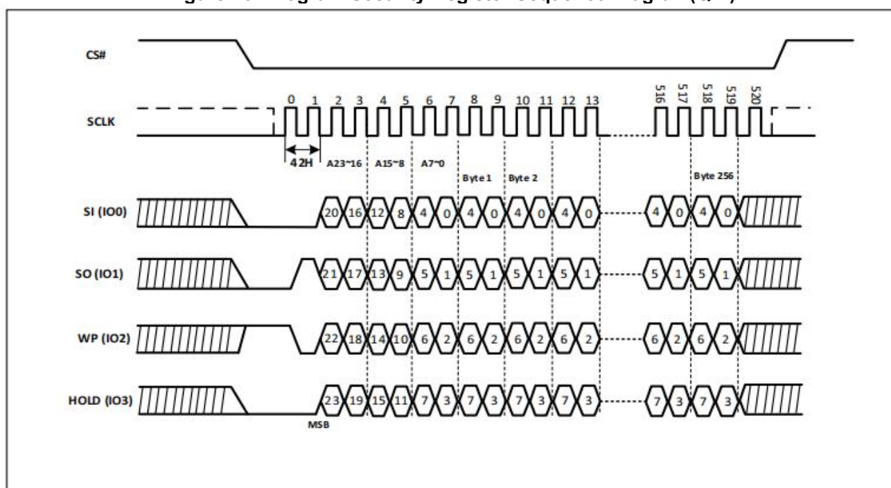
Figure-49. Program Security Register Sequence Diagram(QPI)
