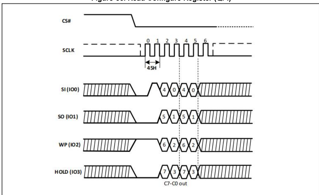
Figure-55. Read Configure Register (QPI)
