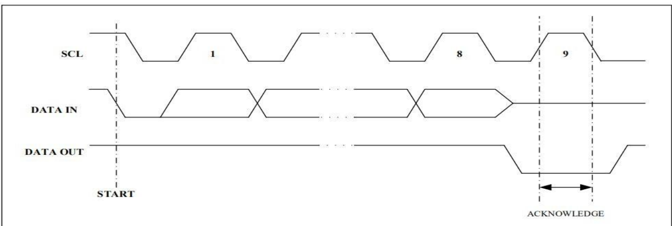
Figure 4. Output Acknowledge
