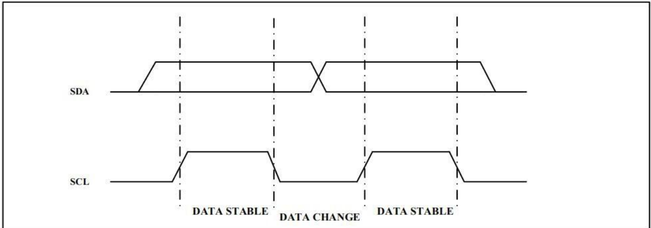
Figure 2. Data Validity
