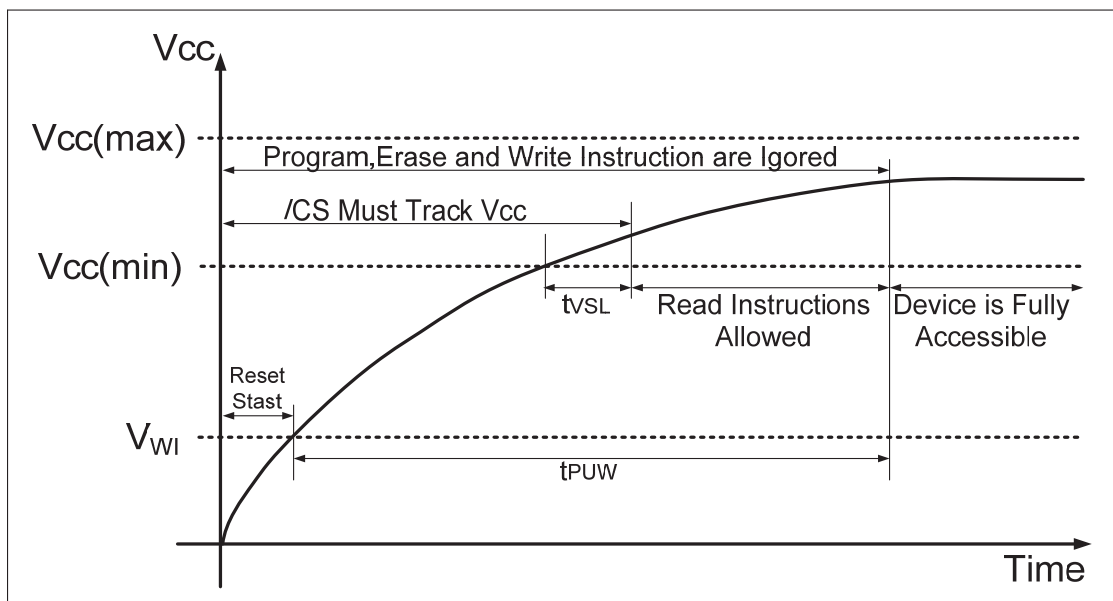
Figure 44, Power-up Timing
